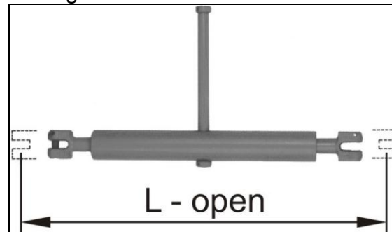
Picture 40: Turnbuckle with short handle to avoid overloading by 50 daN hand force (achieved tension should not be more than 50% LC).
